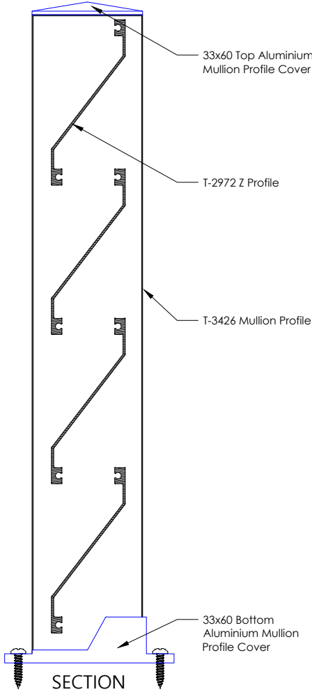
SECTION
