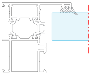
TH62 - 01 Frame Profile
