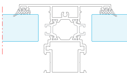
TH62 - 21 Transom Mullion Profile
