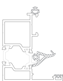
TH62 - 43 Outward Opening Door Adapter Profile
