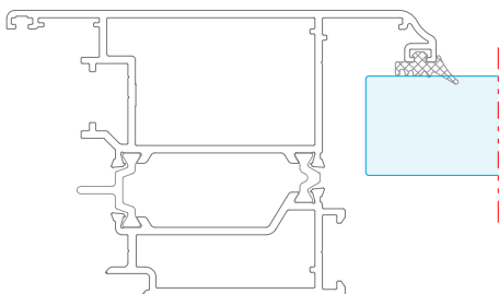
TH62 - 16 Outward Opening Door Sash Profile
