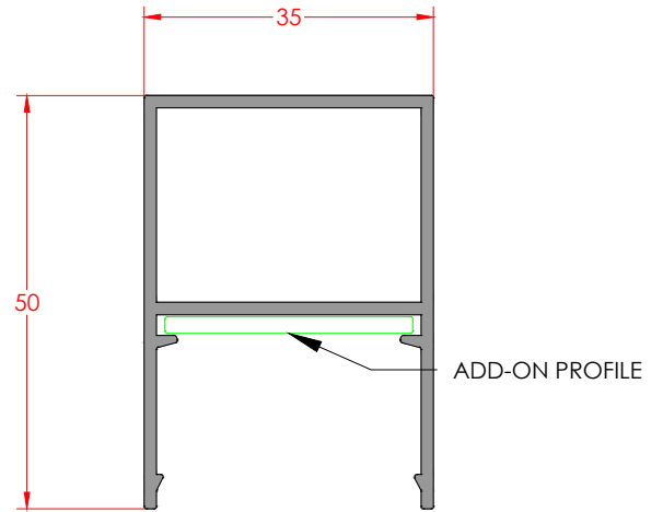
DA35-LONG PROFILE Profile Code: E-DA-352-0- Weight/mt: 0,686
