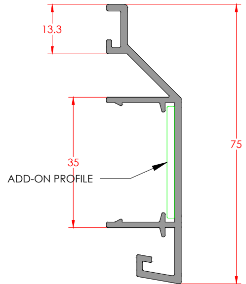
DA75 PROFILE Profile Code: E-DA-75-0- Weight/mt: 0,694
