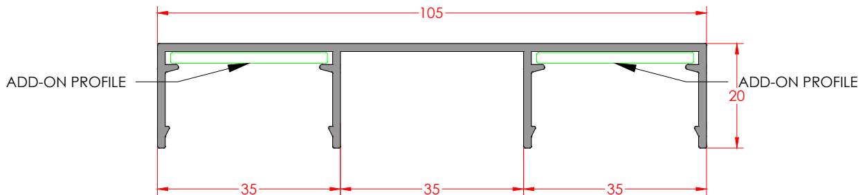
DA105 PROFILE Profile Code: E-DA-105-0- Weight/mt: 0,767
