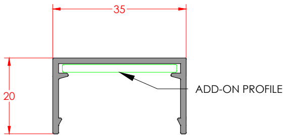
DA35-SMALL PROFILE Profile Code: E-DA-35-0- Weight/mt: 0,311
