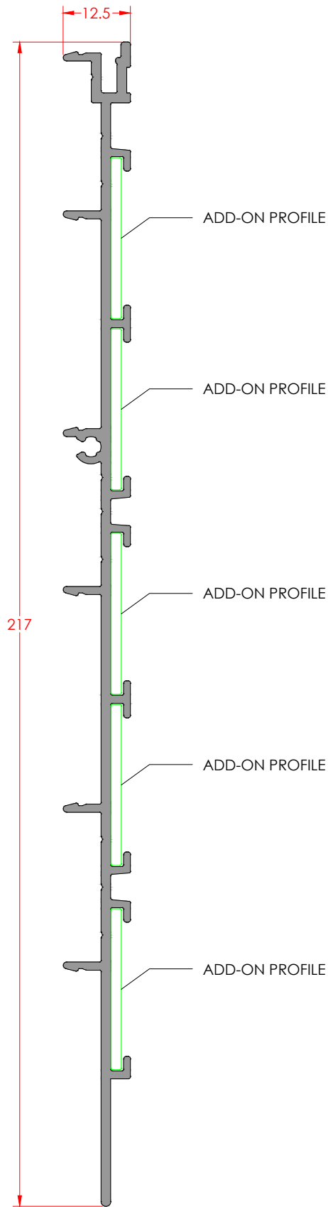
3 PROFILE - BODY Profile Code: E-DA-217-0- Weight/mt: 1,504
