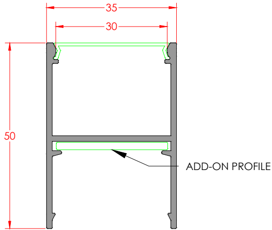
DA35L PROFILE (LED APPLICATION) Profile Code: E-DA-35L-0- Weight/mt: 0,583
