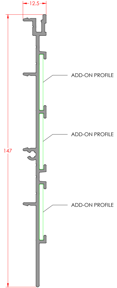
2 PROFILE - BODY Profile Code: E-DA-147-0- Weight/mt: 1,032
