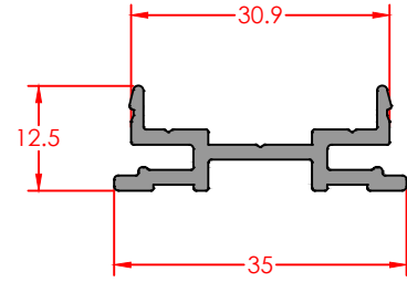
TRANSITION PROFILE Profile Code: E-DA-30-0- Weight/mt: 0,343
