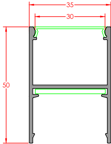
LED APPLICATION COVER PROFILE Profile Code: E-DA-35L-0- Weight/mt: 0,583
