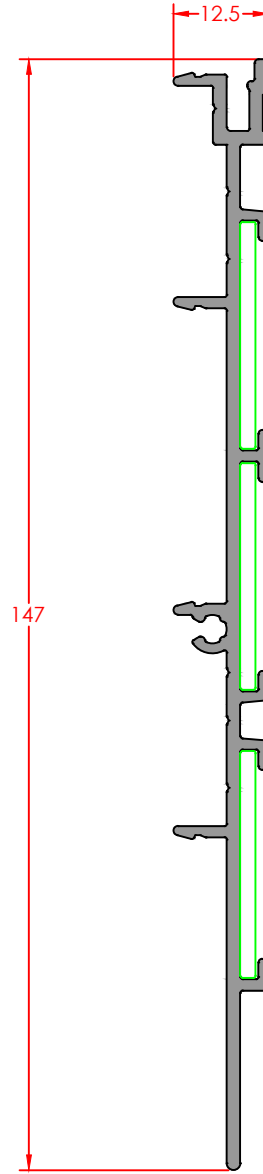
2 AXLE BODY PROFILE Profile Code: E-DA-147-0- Weight/mt: 1,032
