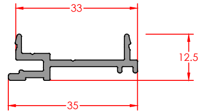
TRANSITION PROFILE Profile Code: E-DA-33-0- Weight/mt: 0,294
