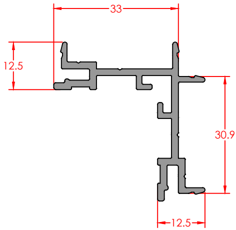
90° CORNER PROFILE Profile Code: E-DA-33C-0- Weight/mt: 0,599
