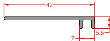
ENDING PROFILE Profile Code: E-DA-42-0- Weight/mt: 0,203
