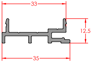
STARTED PROFILE Profile Code: E-DA-33S-0- Weight/mt: 0,313
