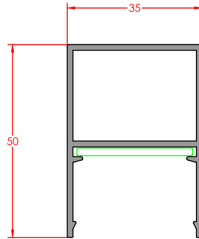
COVER PROFILE Profile Code: E-DA-352-0- Weight/mt: 0,686
