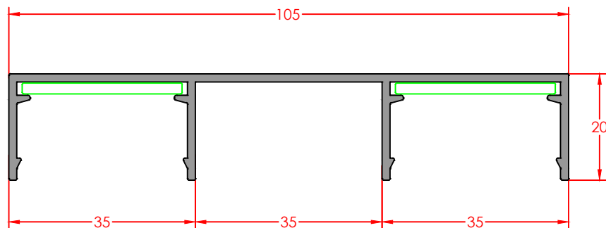
SIDE COVER PROFILE Profile Code: E-DA-105-0- Weight/mt: 0,767
