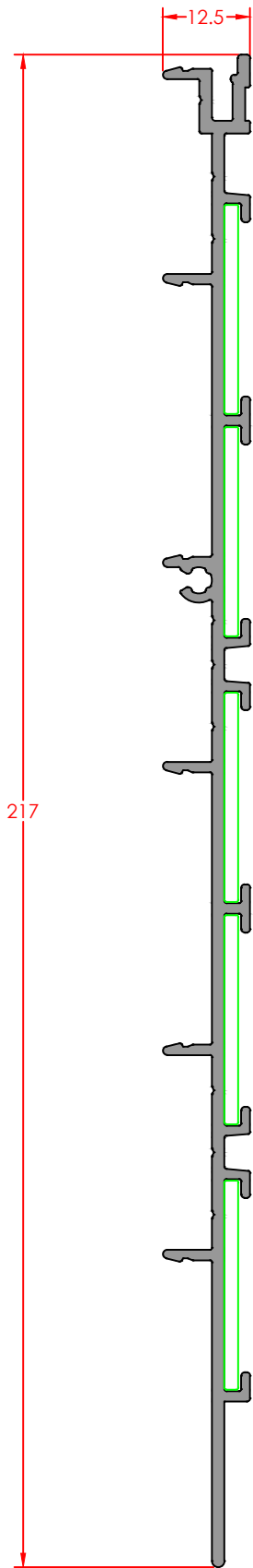
3 AXLE BODY PROFILE Profile Code: E-DA-217-0- Weight/mt: 1,504
