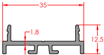
FINISHED PROFILE (4 mm) Profile Code: E-DA-35-0- Weight/mt: 0,301
