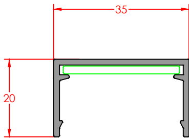
COVER PROFILE Profile Code: E-DA-35-0- Weight/mt: 0,311
