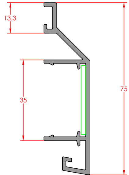
HORIZONTAL COVER PROFILE Profile Code: E-DA-75-0- Weight/mt: 0,694
