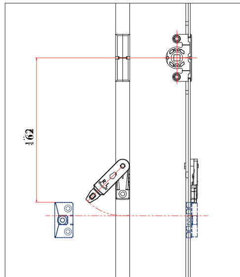
Locking Plate for T-10189-50-0-1 (9 mm) T-19050-09-0-1
