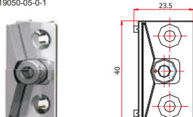
Locking Plate for Thyssen for T-10189-50-0-1 T-19050-05-0-1
