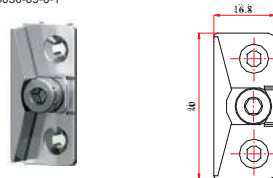
Locking Plate for Thyssen for T-10189-50-0-1 T-19050-05-0-1
