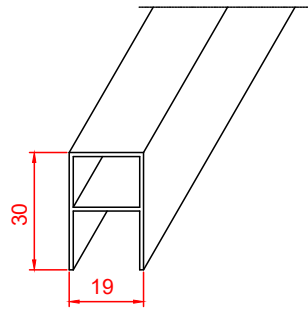
T-743120-00-0-0 Aluminium Frame Profile
