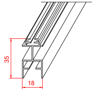
T-743121-00-0-0 Aluminium Sash Profile
