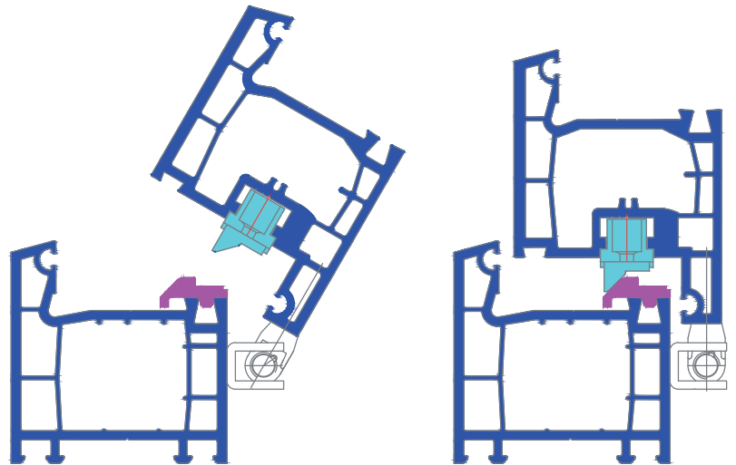
Middle Hinge Concealed, 13 mm
